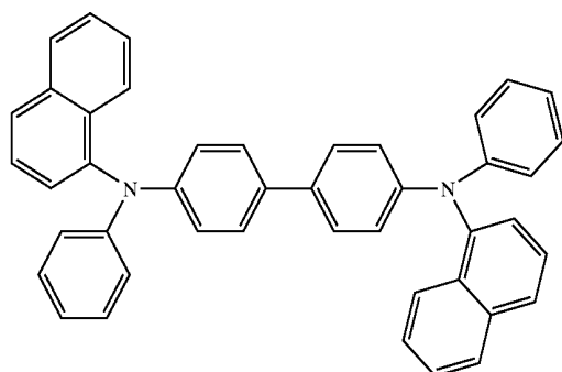
NPB
